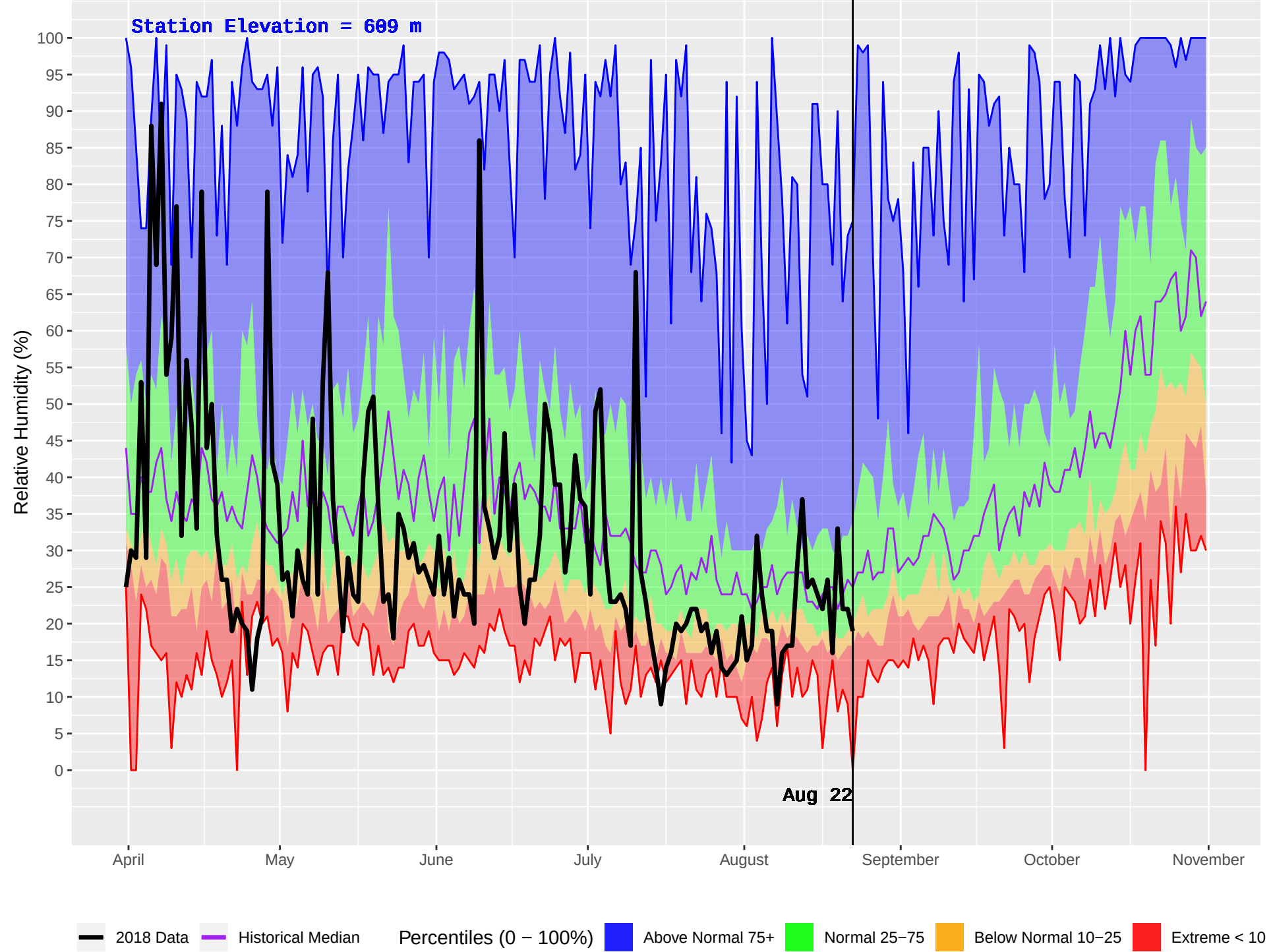
ROCK CREEK (394) : Historical (1990–2016) and Current (2018) Daily Relative Humidity
