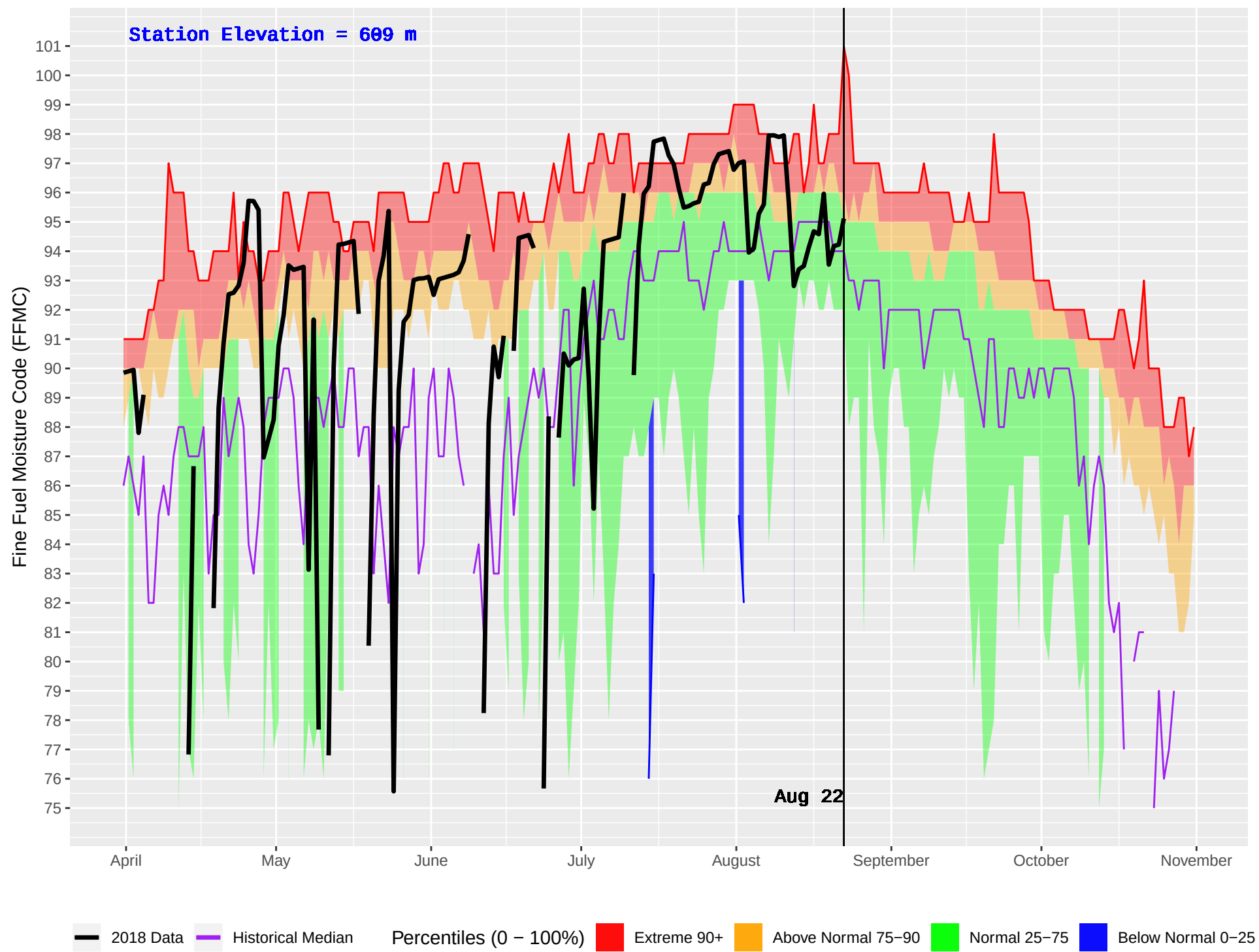
ROCK CREEK (394) : Historical (1990–2016) and Current (2018) Daily Fine Fuel Moisture Code (FFMC)
