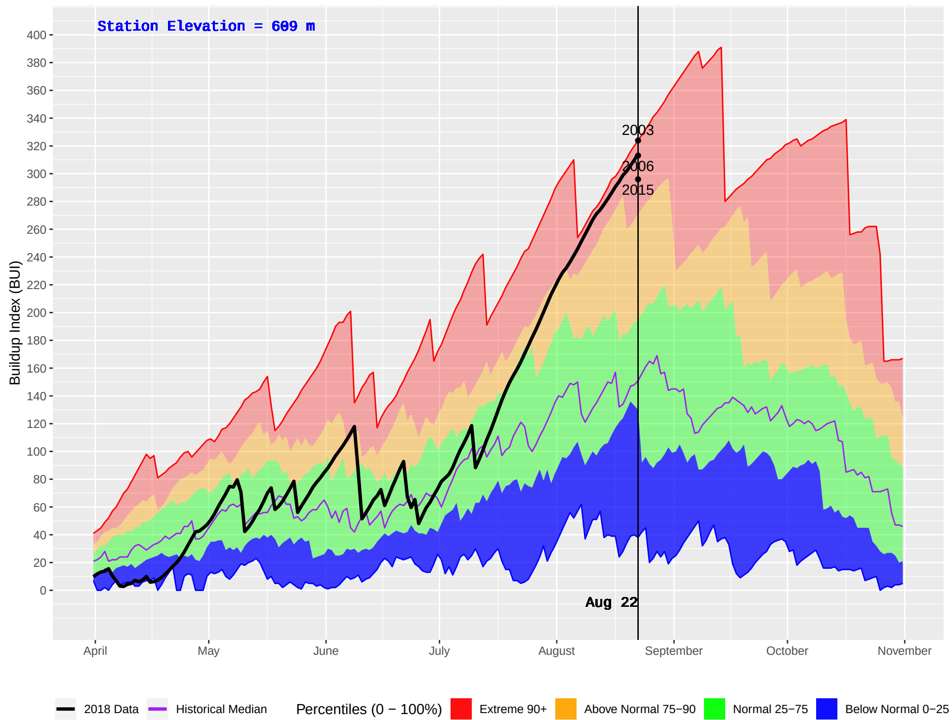
ROCK CREEK (394) : Historical (1990–2016) and Current (2018) Daily Buildup Index (BUI)
