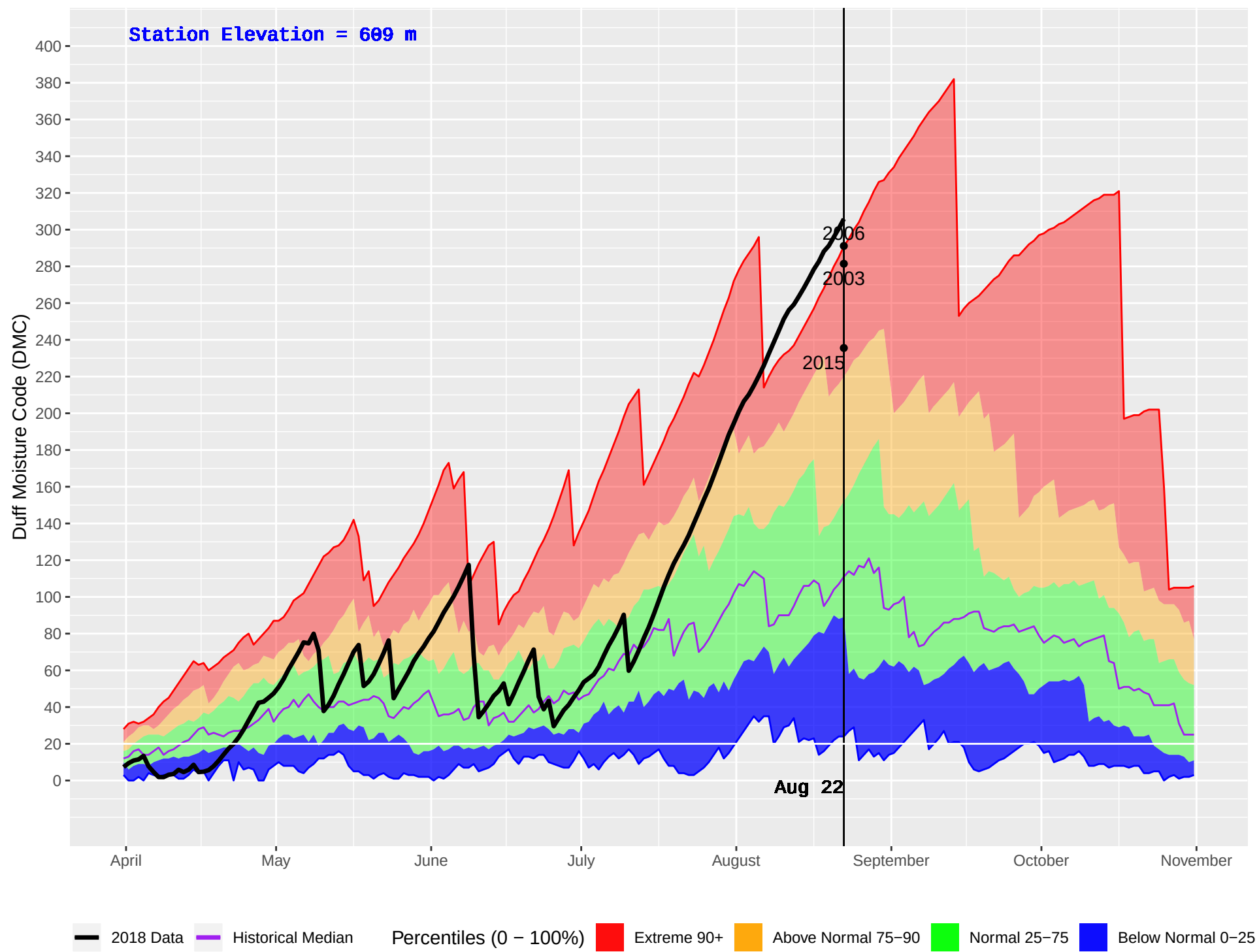
ROCK CREEK (394) : Historical (1990–2016) and Current (2018) Daily Duff Moisture Code (DMC)
